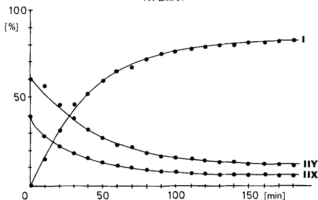
Fig. 2. Reversible isomerisation of valofan diastereoisomers IIX and IIY to proxibarbal (I) in aqueous solution at pH 7.4 and 37°
