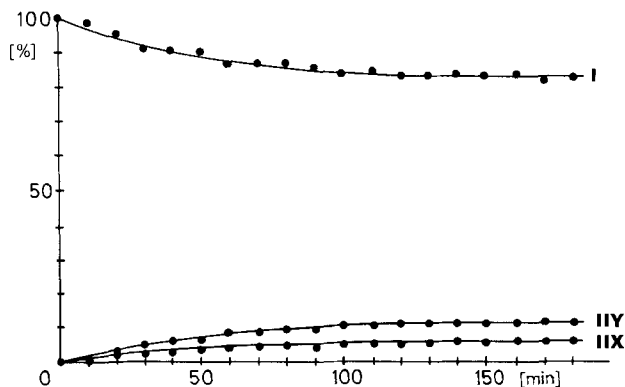
Fig. 1. Reversible isomerisation of proxibarbal (I) to valofan diastereoisomers IIX and IIY in aqueous solution at pH 7.4 and 37°
